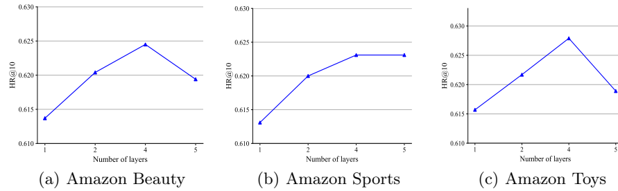
Fig. 5: Impact of knowledge extractor depth.
