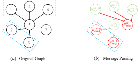
Fig. 3: (a) The items in the orange and blue dashed boxes are the out-degree and in-degree neighbors; (b) The red and green dashed circles indicate the out-degree and in-degree features, respectively.
